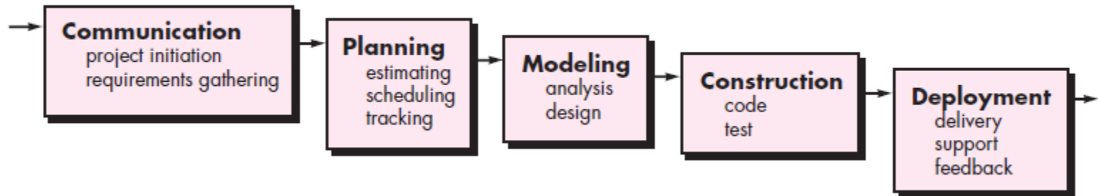
FIGURE 2.3 The waterfall model
