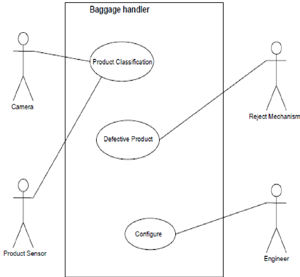
FIGURE 3.3 Use case diagram of the baggage inspection system.
